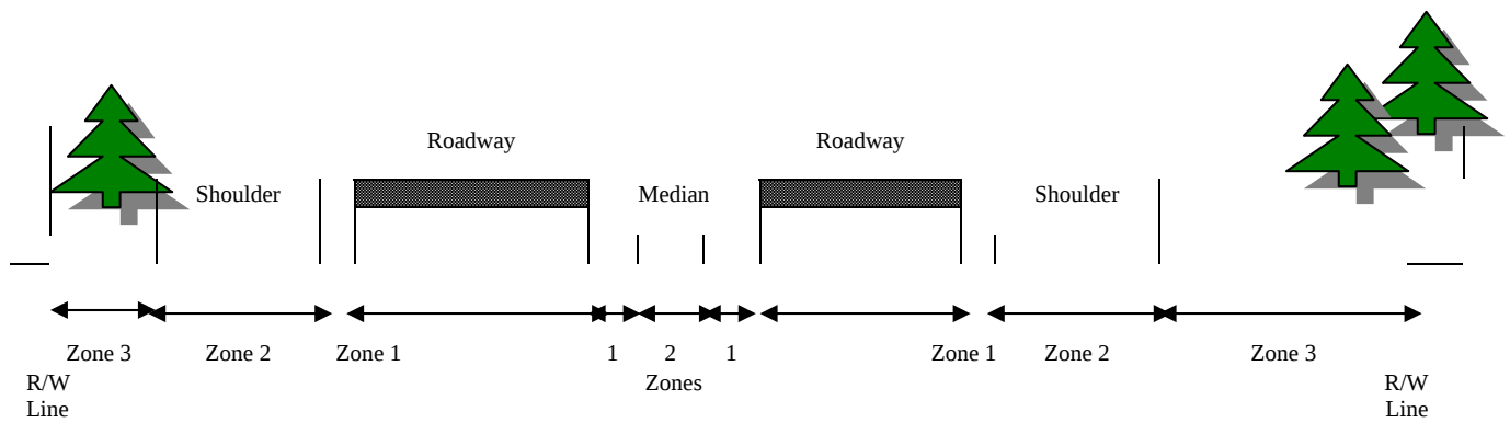
Figure 5: Cross Section Freeway Zone I-84 Cascade Locks Hwy I-84 20
